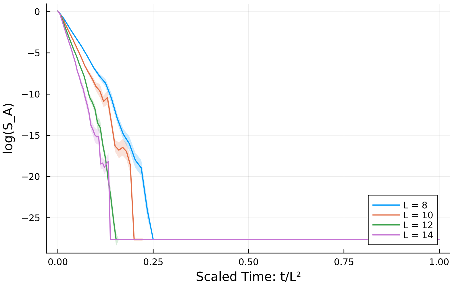
Scaled Log Entropy Evolution ( p = 0.783333 )
